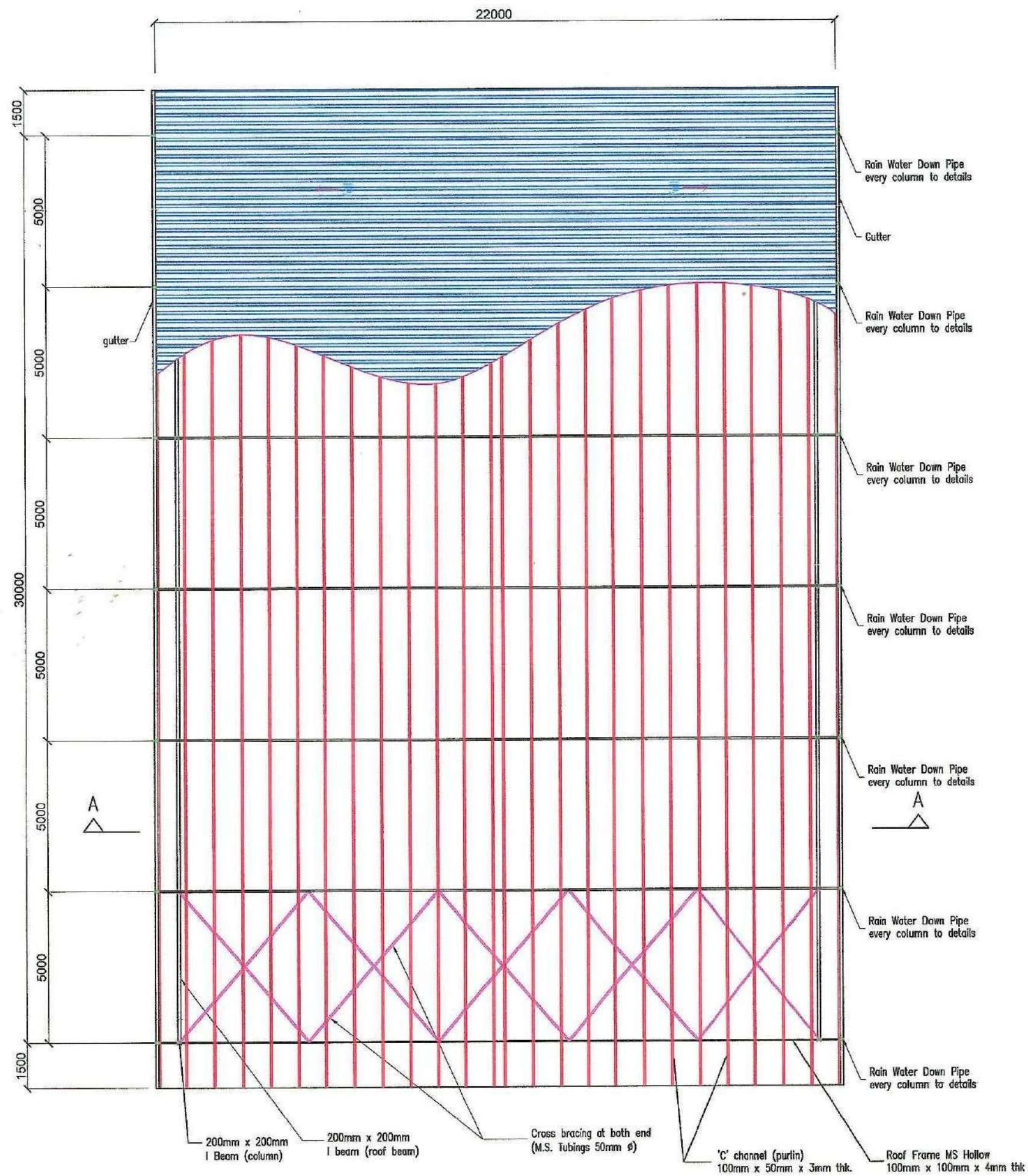
ROOF PLAN
