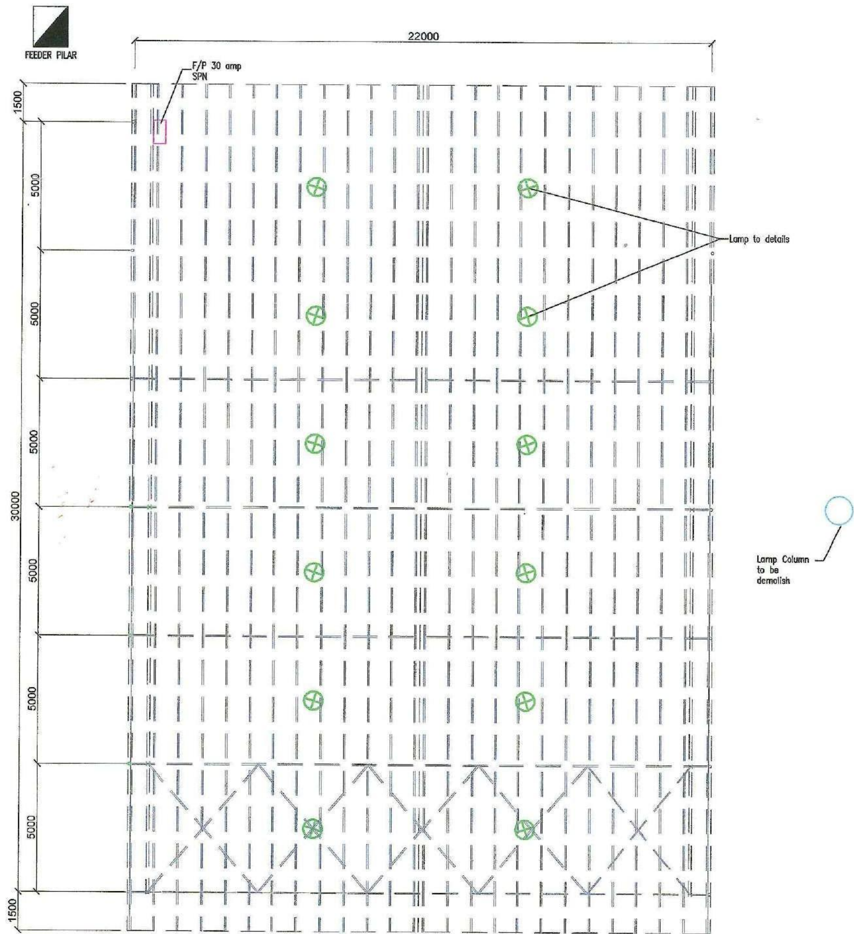
LAMP PLAN LAYOUT
